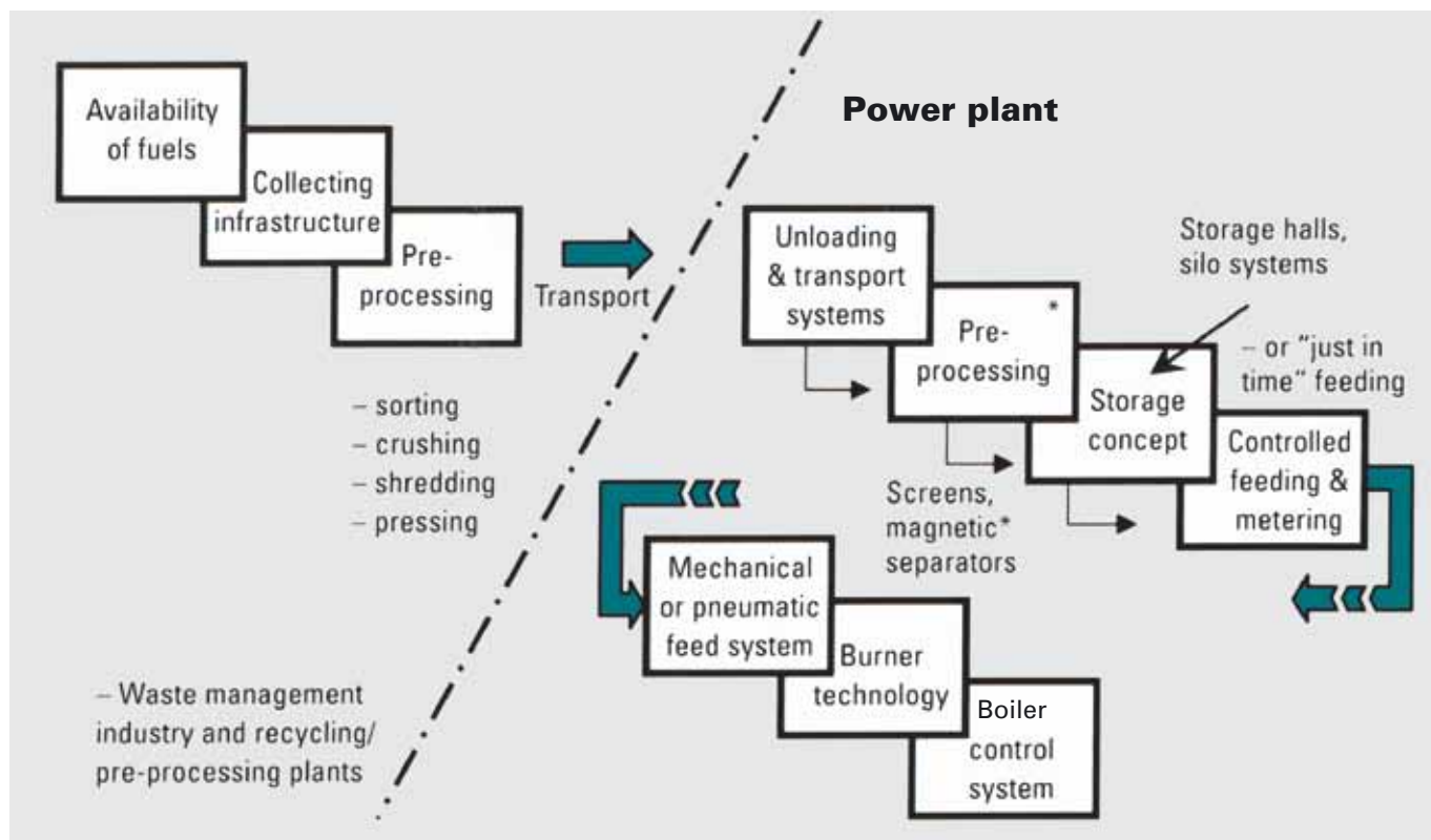
Fig.2 Diagram showing utilisation of alternative fuel
