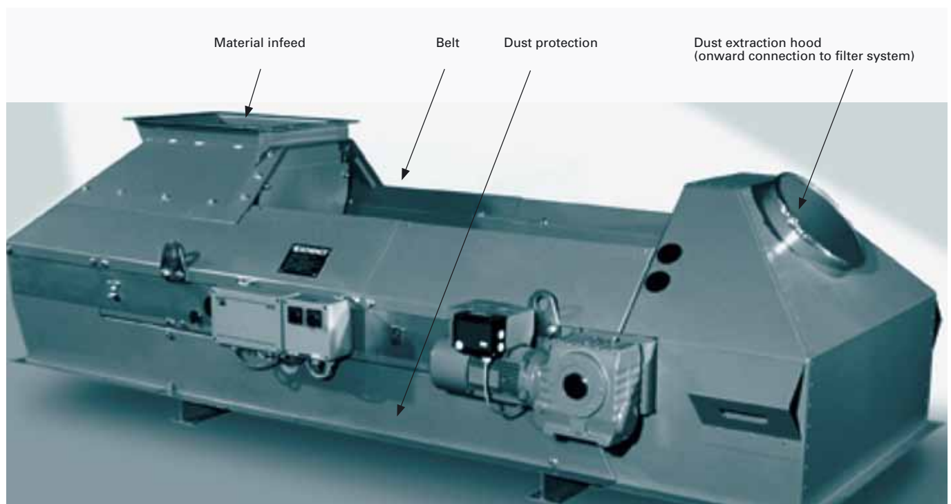
Fig. 11 MULTIDOS® weighfeeder
